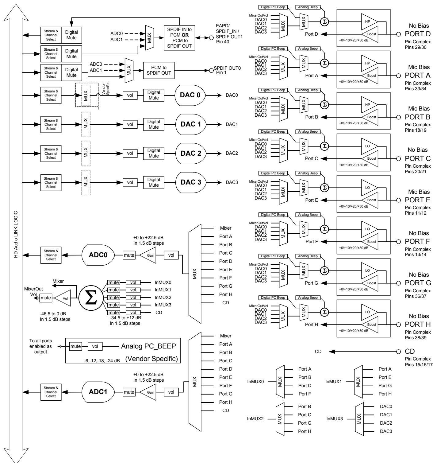
Figure 11. 40QFN Functional Block Diagram
